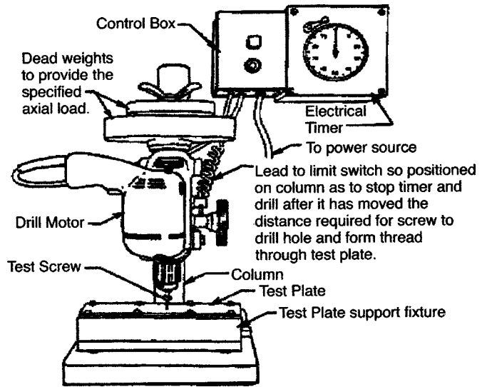
FIG. 2 Drill-Drive Test Apparatus
